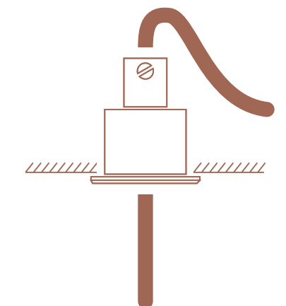
Ø 41 x 46,5 mm WL1-ZBS2.06
