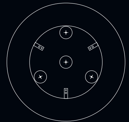
BALDACHIN / CANOPY DURCHMESSER 520MM / HÖHE 40MM DIAMETER 520MM / HEIGHT 40MM
